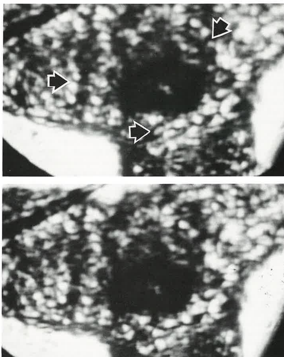
Figure 3. Two frame enlargements from the videomicrograph of Brownian movement in Clarkia pollen, demonstrated at INTER/MICRO-92. Three areas where clear differences may clearly be seen are indicated by arrows. Scale bar = 10\ \mu\text{m} . Zones within these pollen cells were shown to be in a continual state of agitation, exactly as described by Brown in his account from June 1827.
